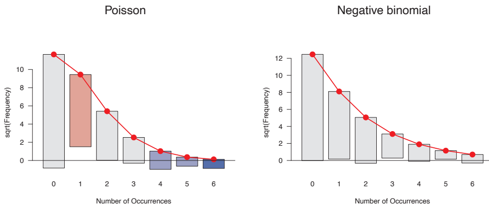
Figure 3.16: Hanging rootograms for the Federalist Papers data, comparing the Poisson and negative binomial models. {fig:Fed0-Fed1}
