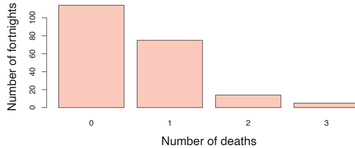
{fig:cyclists2} Figure 3.6: Frequencies of number of cyclist deaths in two-week periods in London, 2005–2012.
