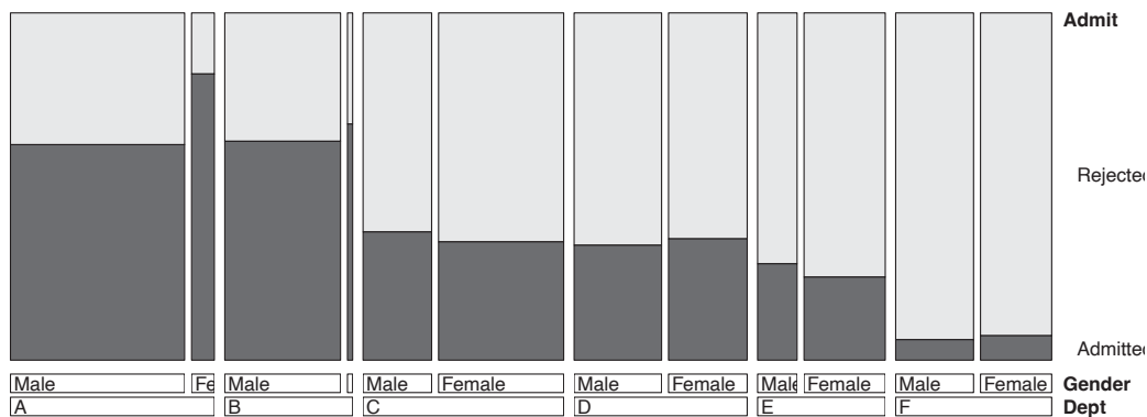
Figure 5.34: Doubledecker plot for the UCBAmissions data.
